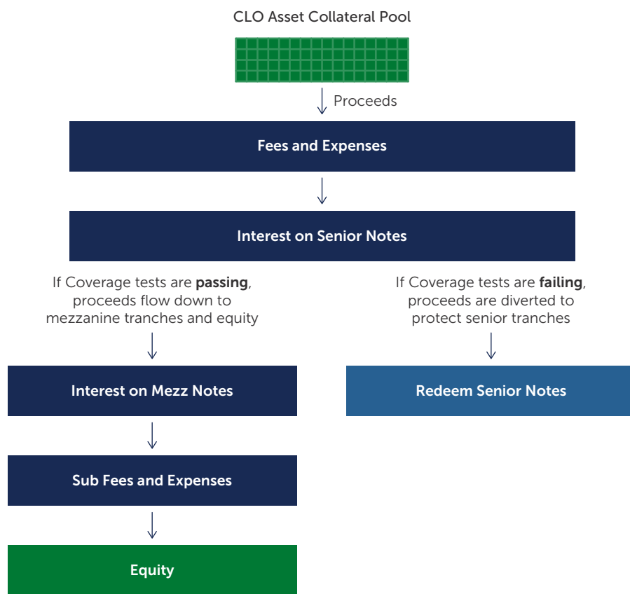
Figure 2: CLO Waterfall
